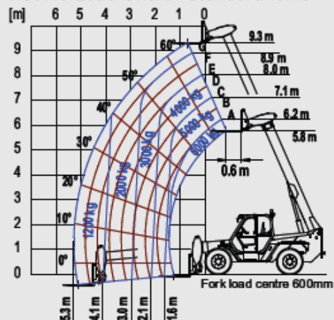
P60.10 Load Chart - Standard forks
