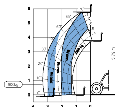
Lift capacity chart with floating forks (L 1200 mm-section 100 x 40 mm)****
