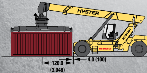
20'-0 END ON LIFTING CAPACITIES
