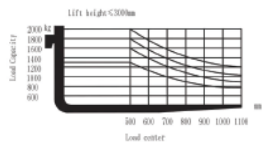
Load chart
