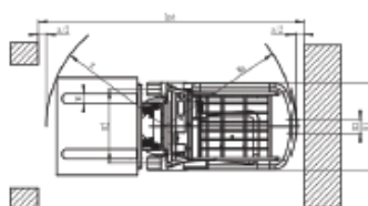
2000mm Safety clearance 1400mm
