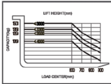
LOAD CHART
