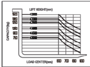
LOAD CHART
