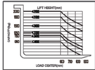
LOAD CHART
